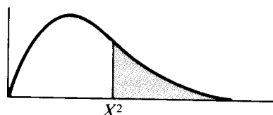
Chi-Square Distribution
