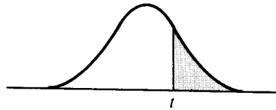
Student's t -distribution
