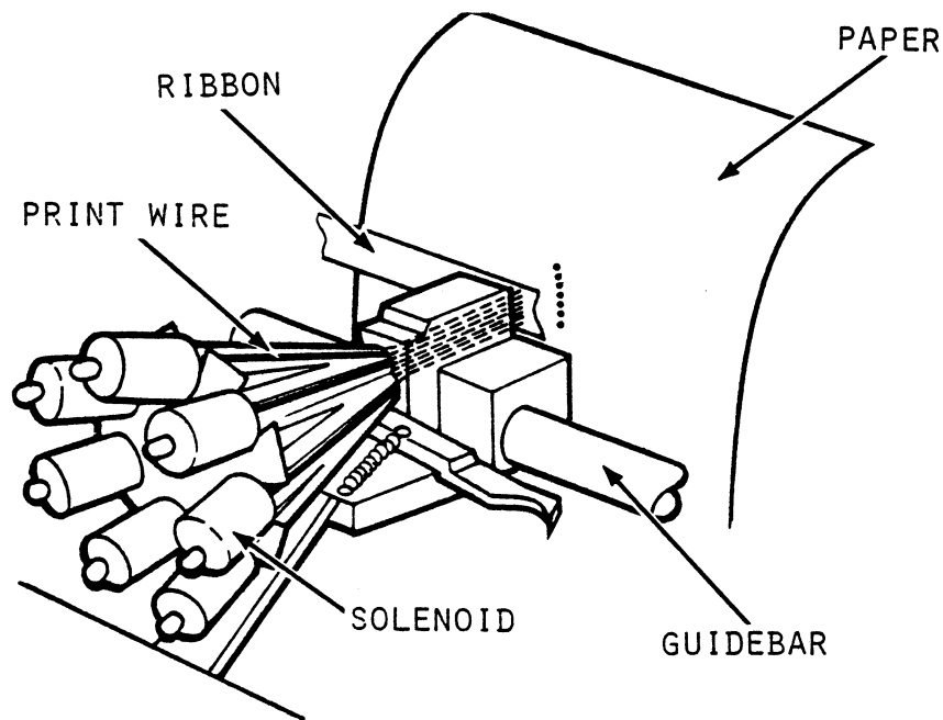
Figure 4-2. Print Head Assembly
