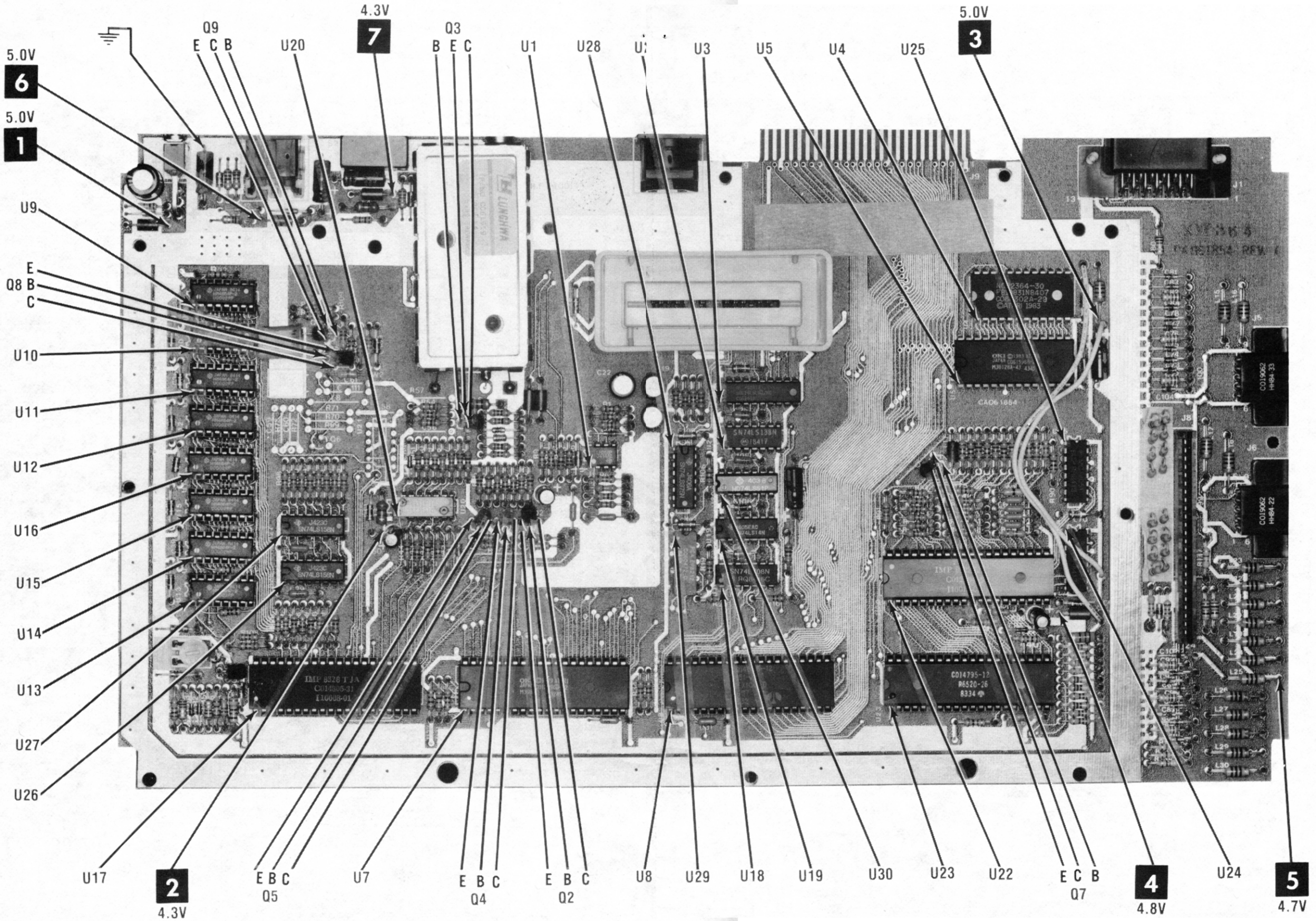
ARROWS ON IC'S INDICATE PIN 1 UNLESS NOTED
