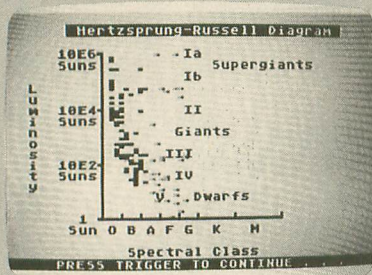
Hertzsprung-Russell Diagram
