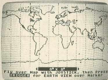
Mercator Projection
