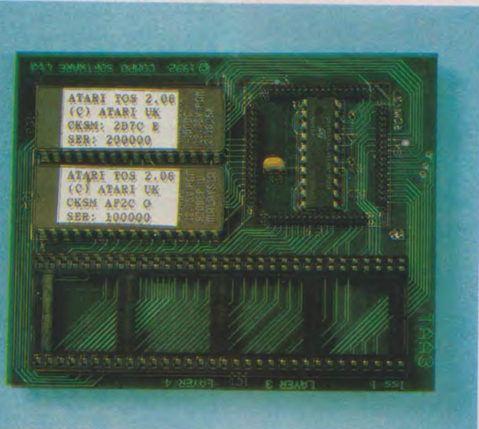
The STE has a square 68000, so a different board is required. Note the ability to add STFM standard extra boards.
