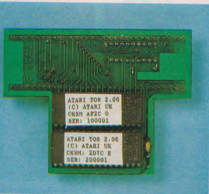
The official TOS 2.06 upgrade for the STFM is soldered over the existing 68000 CPU and allows for additional boards to plug in on top.
