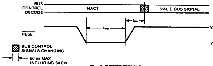
Fig. 8 RESET TIMING
