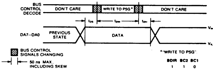
Fig. 10 WRITE DATA TIMING
