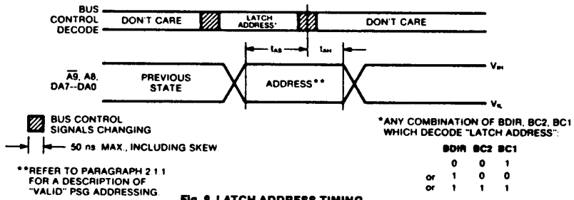
Fig. 9 LATCH ADDRESS TIMING
