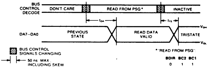
Fig. 11 READ DATA TIMING
