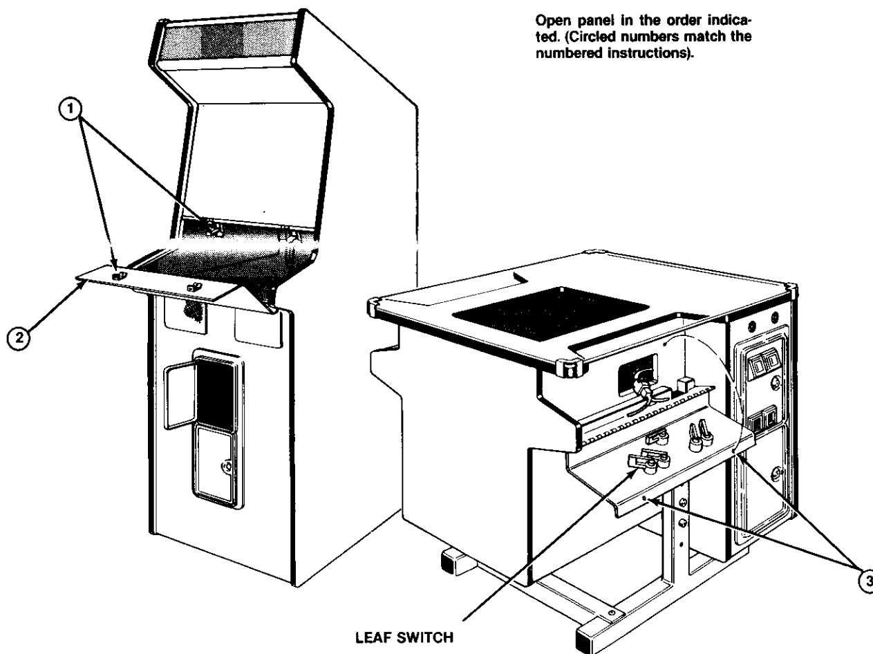
Figure 3-2 The Control Panel
