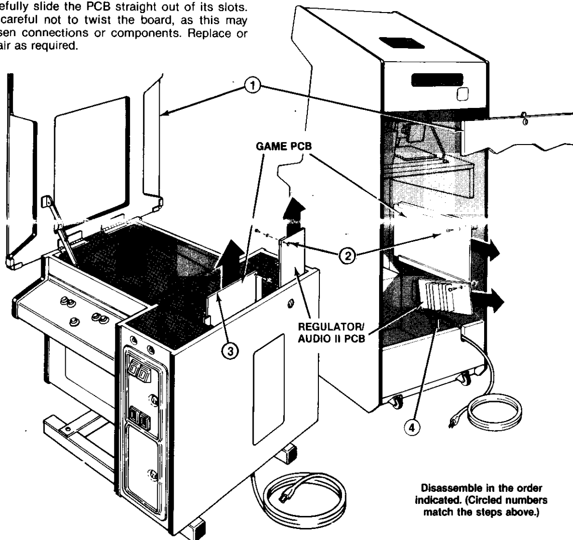
Figure 3-7 Printed-Circuit Board Removal
