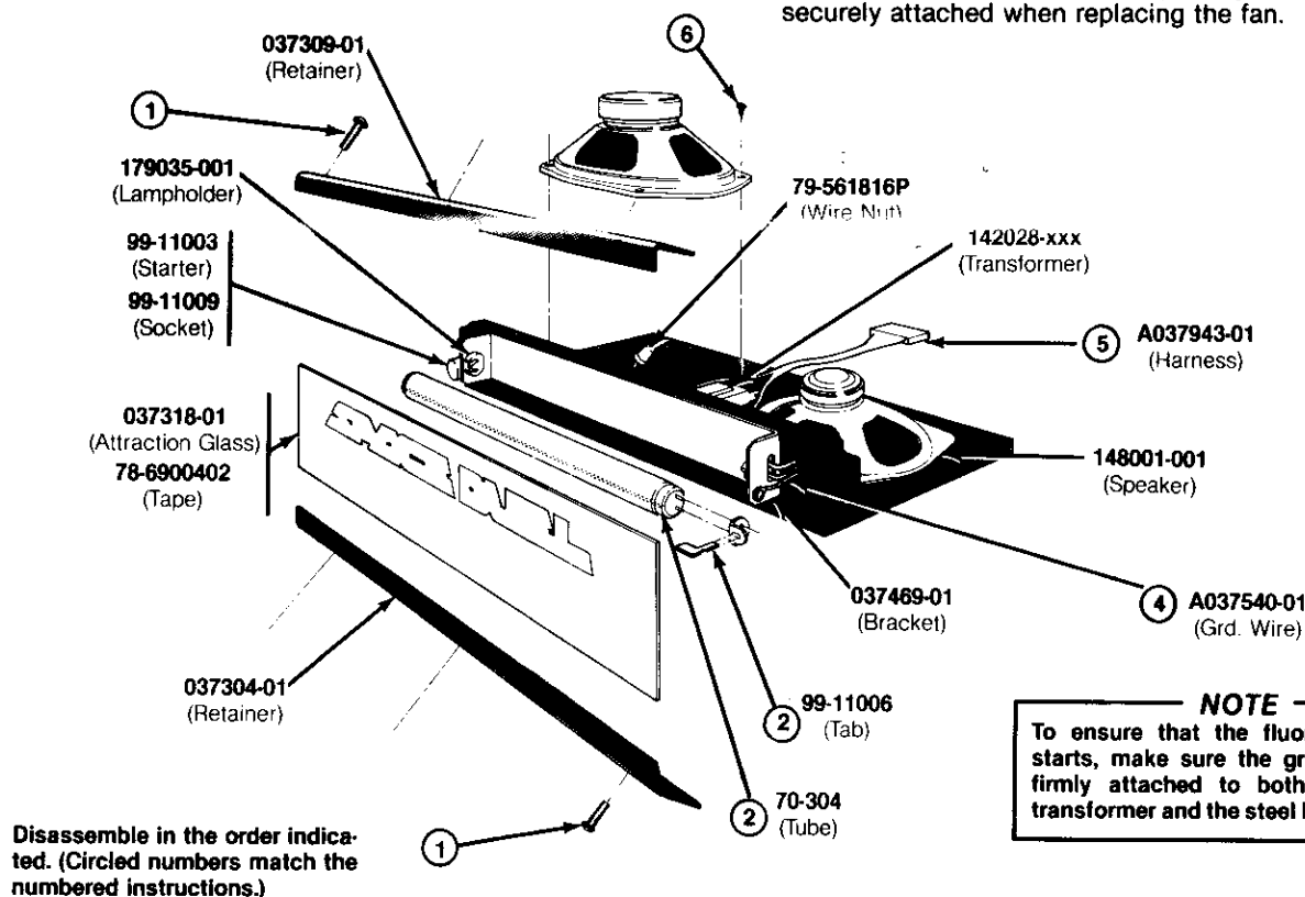
Figure 3-4 Speaker, Fluorescent Tube and Fan
