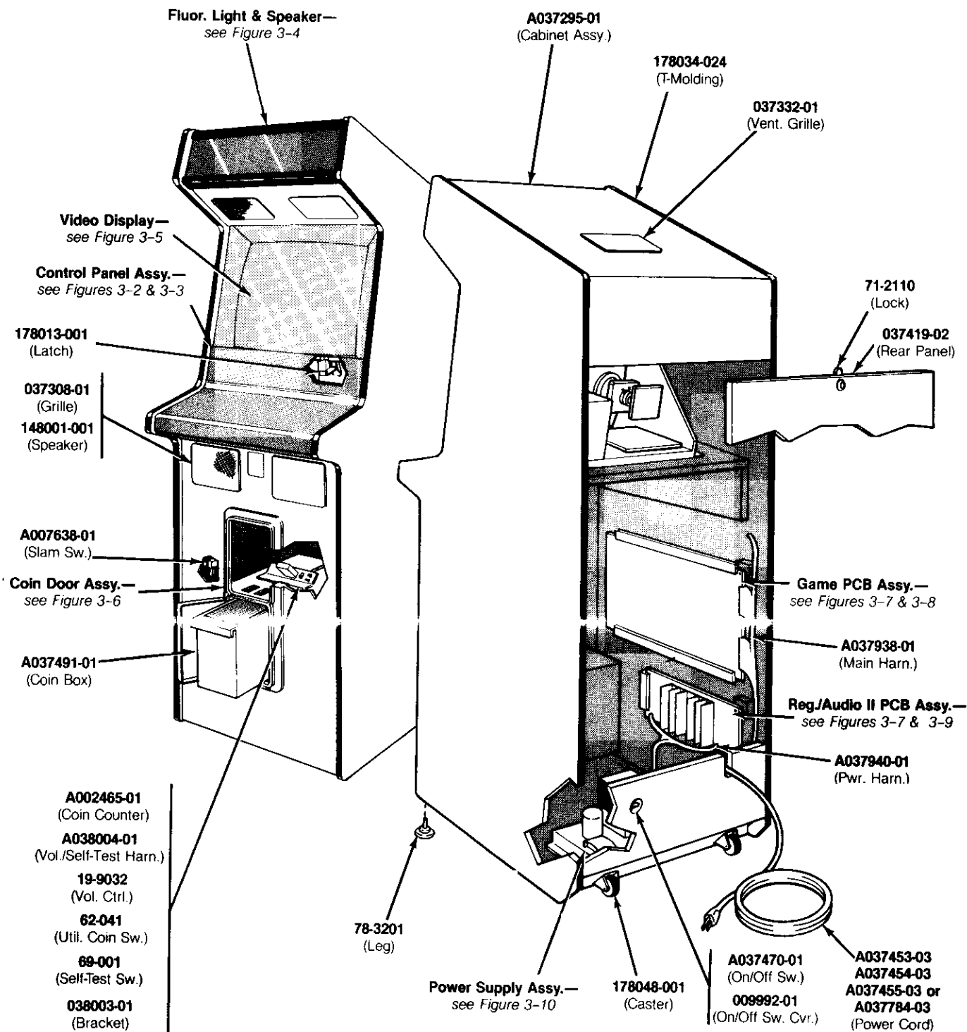
Figure 3-1 Upright Cabinet-Mounted Assemblies A037294-xx A
